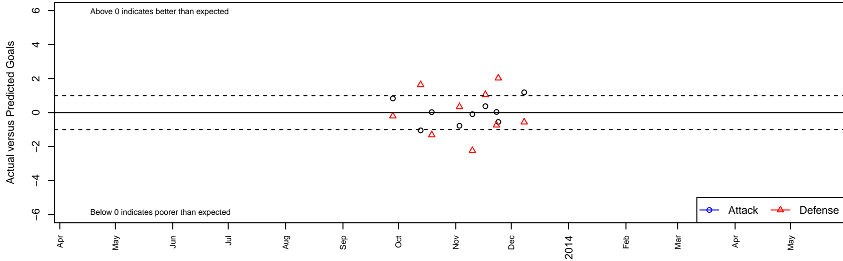
Lobitos B01 Dots are actual minus expected GF (blue circles) and GA (red triangles). Blue line is smoothed change in attack strength. Red is smoothed change in defense strength.
